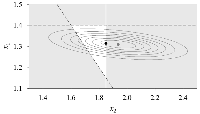
Fig. 1 Isolines of the objective function (black ellipses) and constraints (straight lines) of an ICLS problem. The optimal OLS solution (gray dot) is in the infeasible region (gray shaded area). The ICLS solution (black dot) is the projection of the unconstrained solution onto the boundary of the feasible set. One constraint is active in the optimal solution (solid line) and two are inactive (dashed lines).
