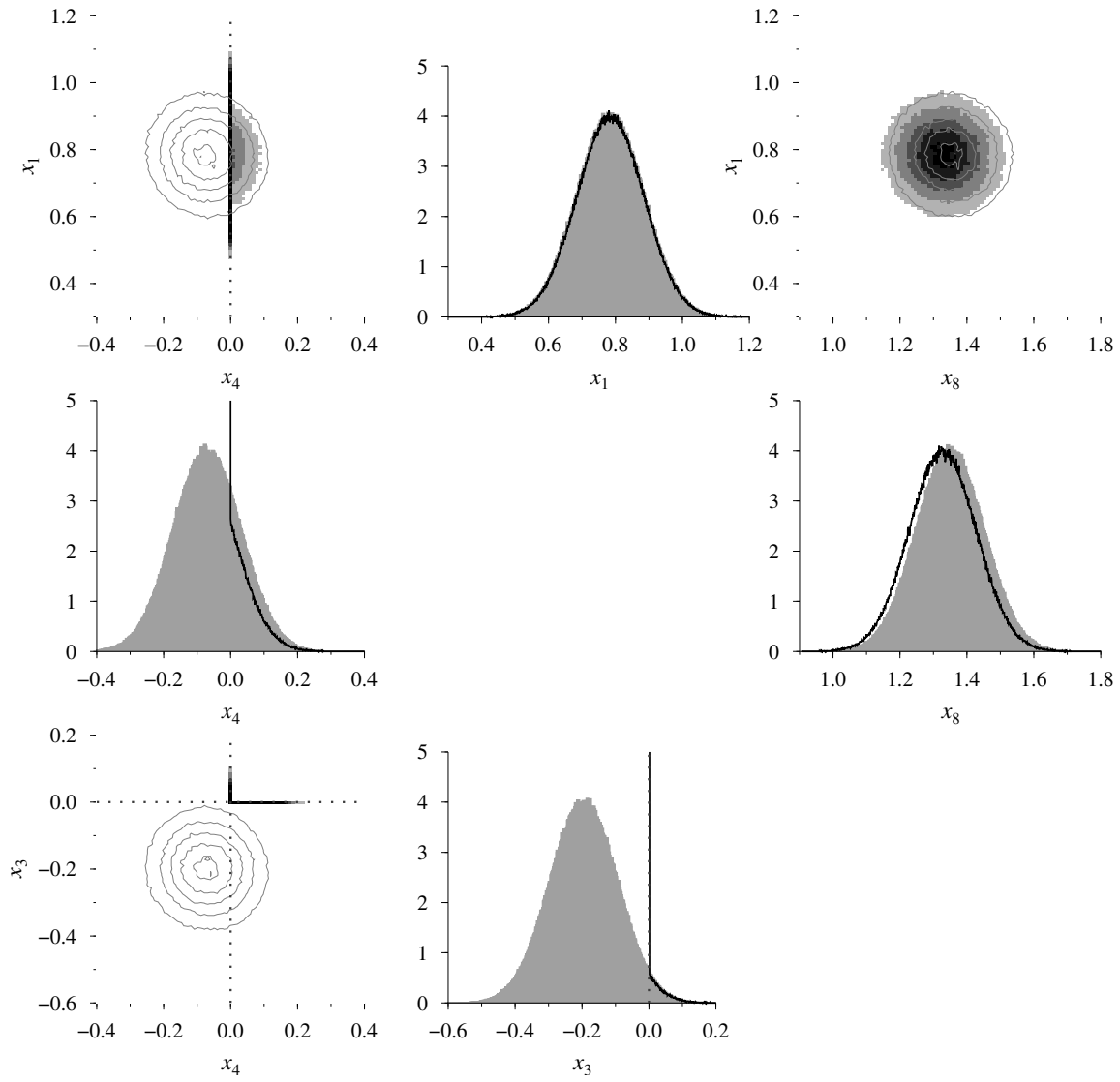
Fig. 7 Probability density functions (joint and marginal) of the positive cosine function estimation problem. Three different pairs of joint PDFs are shown: x_3 & x_4 , x_4 & x_1 and x_1 & x_8 . The contour lines are from the OLS estimate and the dotted lines are the constraints. These pairs show the range of joint PDFs that can be expected from a multi-dimensional estimation problem. While some joint PDFs are entirely in the feasible region, some of them are either partly or entirely in the infeasible region. Due to the negligible correlation between the parameters, all the OLS joint PDFs are near circular.
