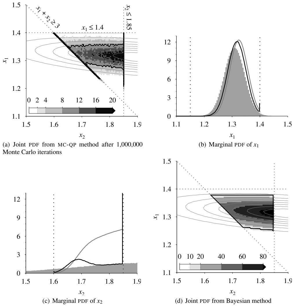
Fig. 5 Probability density functions (joint and marginal) from the line-fitting problem with dependent constraints. From the joint PDFs it is clear that this is a bounded constraint problem as the densities are confined to the triangular region formed by the constraints. Due to the inclined plane x_1 + x_2 \geq 3 , there is complex accumulation of the probability densities taking place in the marginal PDF of x_2 .
