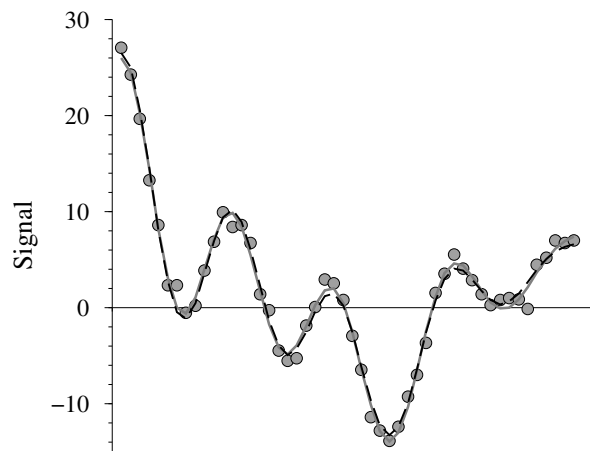
Fig. 6 Observations (gray dots), and the OLS (gray line) and ICLS (black line) fits to the observations of the positive cosine function estimation problem.
