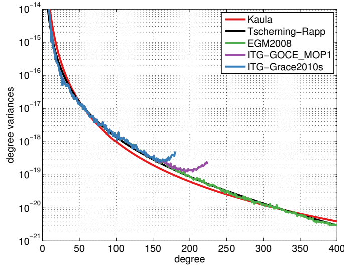
Fig. 1 Comparison of degree variances from model computations (Kaula, Tschering-Rapp) and up-to-date gravity field models from measurements ITG-GRACE2010s and EGM2008 (ICGEM, 2010) in comparison with an unconstrained (only polar gap regularization) internal version of the ESA-GOCE-HPF model GO_CONS_EGM.TIM.2i (Pail et al., 2010).
